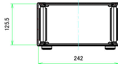
B-B (1:5)
