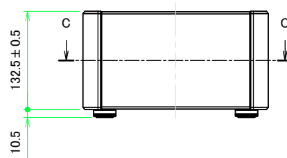
B-B (1:5)
