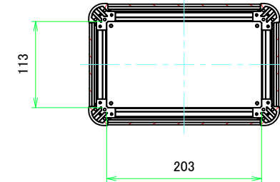
C-C (1:5)
